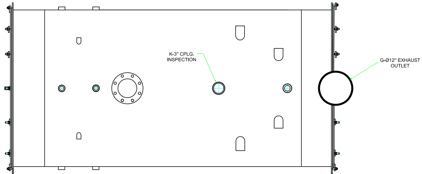
TOP VIEW
